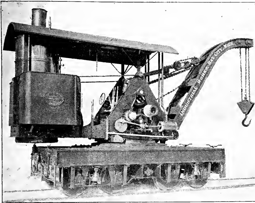
Fig. 209. LOCOMOTIVE CRANE, BUILT BY THE INDUSTRIAL WORKS. Capacity, 12 tons.
